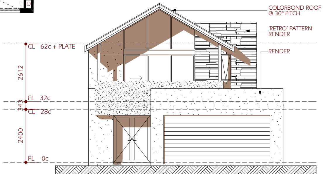
FRONT ELEVATION 1:100
