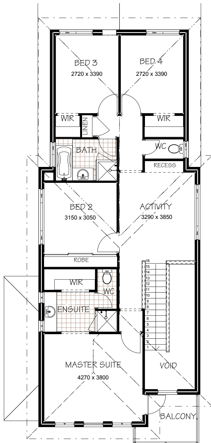
UPPER FLOOR PLAN 1:100
