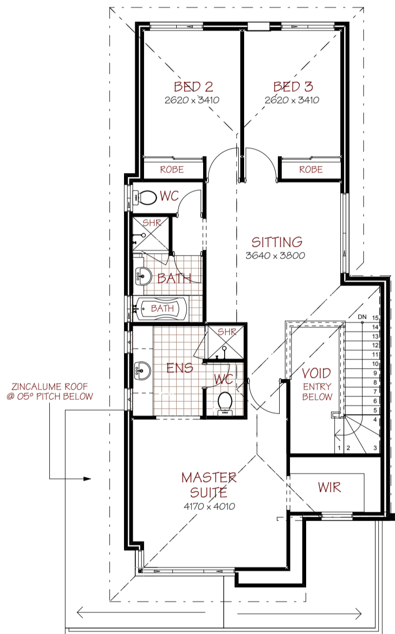
UPPER FLOOR PLAN 1:100
