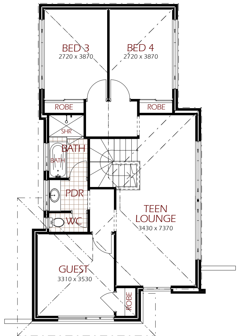
UPPER FLOOR PLAN 1:100
