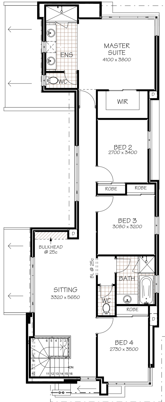
UPPER FLOOR PLAN 1:100
