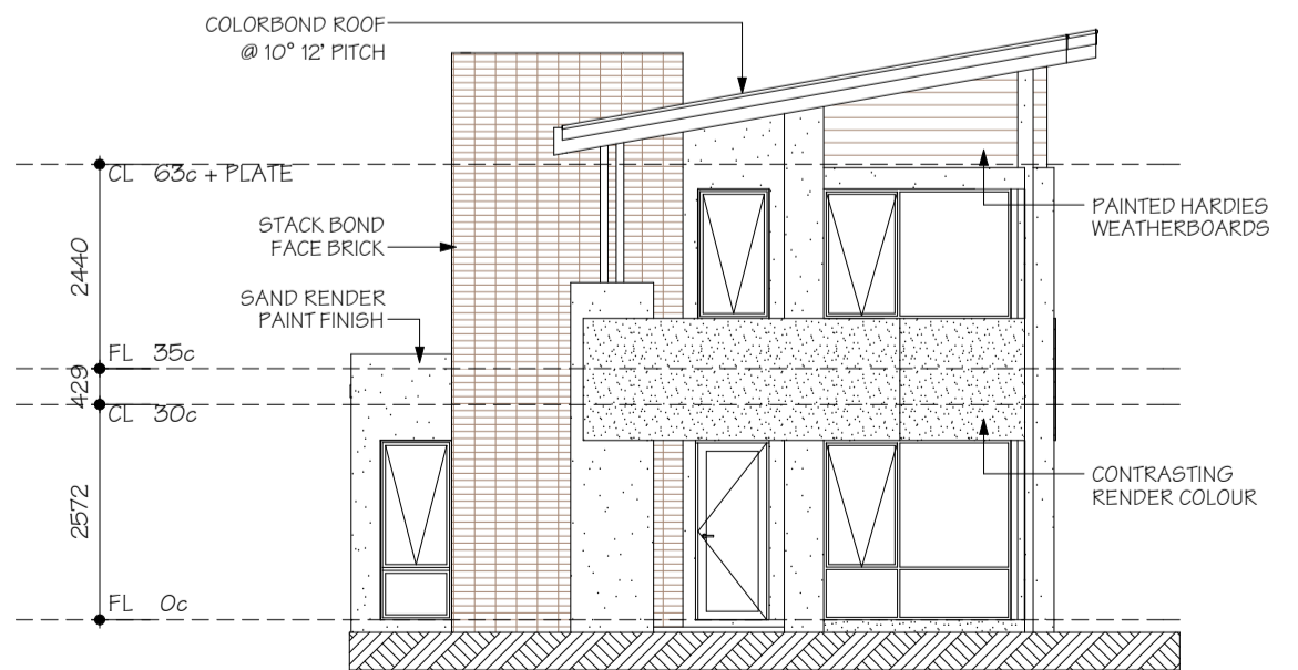
FRONT ELEVATION 1:100
