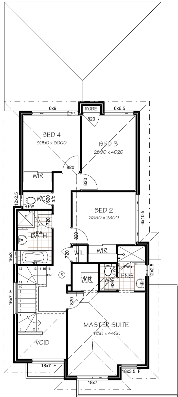
UPPER FLOOR PLAN 1:100
