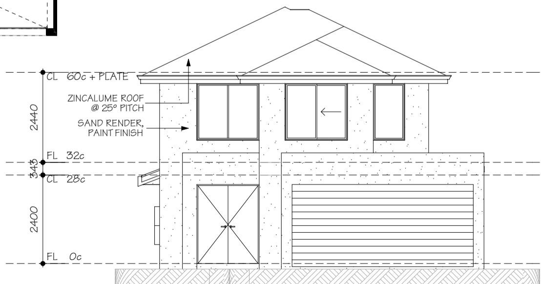
FRONT ELEVATION 1:100
