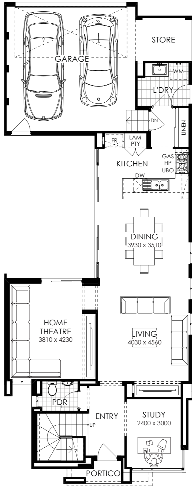
GROUND FLOOR
