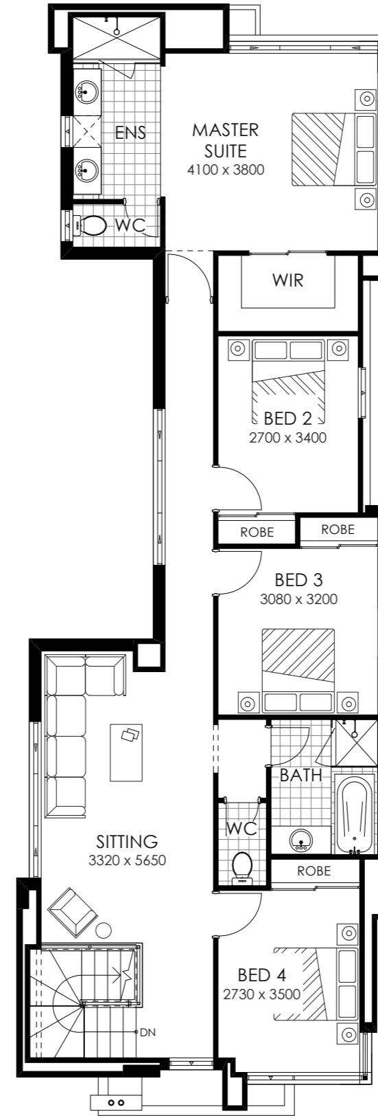
UPPER FLOOR
