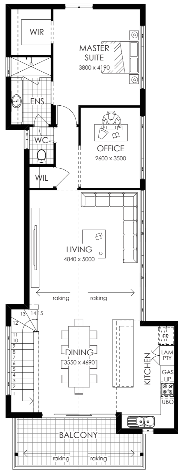
UPPER FLOOR PLAN 1:100
